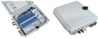
FAT-12A-II 8-Core Optical Cable Distribution Box Size:225*200*65MM
